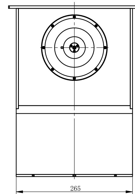
View G
